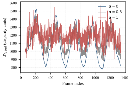
Fig. 2. Fused disparity estimates over four approach-and-retreat cycles for three fusion weights ( \alpha = 0, 0.5 , and 1 )
