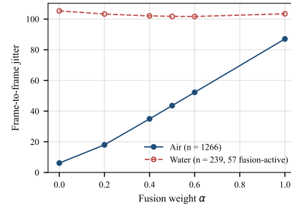
Fig. 3. Frame-to-frame jitter of the fused estimate versus fusion weight \alpha in air and underwater
