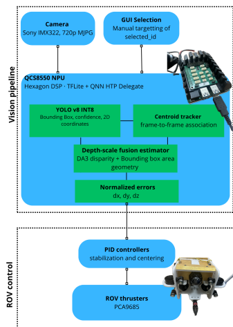
Fig. 1. Overview of the visual stationkeeping pipeline. The perception modules run on the Qualcomm QCS8550 platform, while the PID controller and thruster blocks represent the intended closed-loop system architecture
