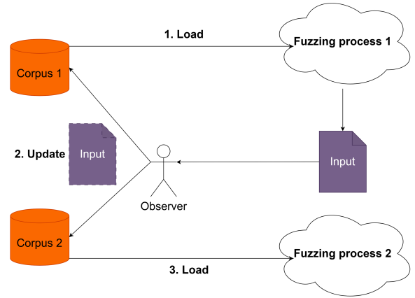
Fig. 2. Corpus-only cooperative execution with independent coverage and learning state
