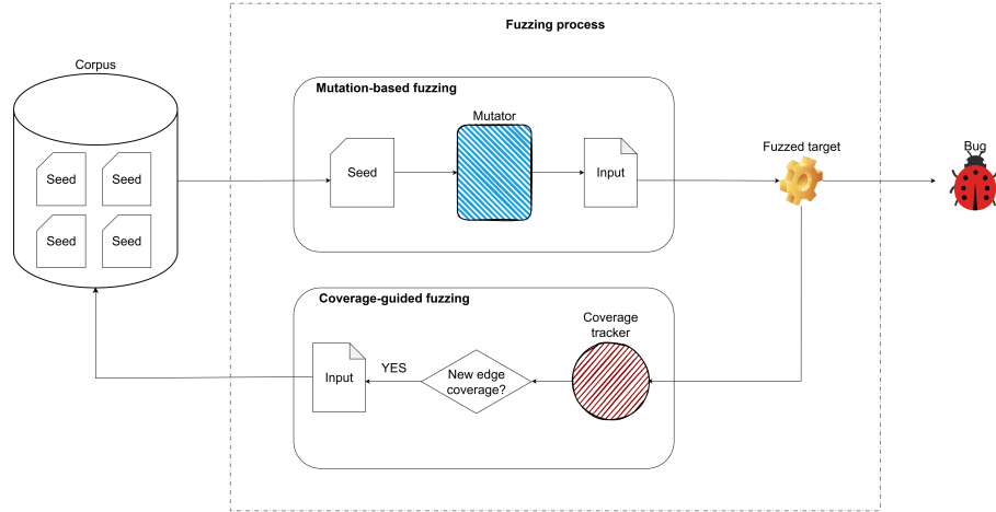
Fig. 1. Mutation-based coverage-guided fuzzing
