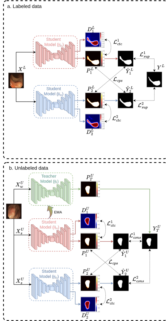
Fig. 1. Overview of the proposed framework
