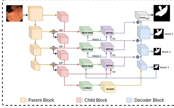
Fig. 2. Overview of the backbone architecture
