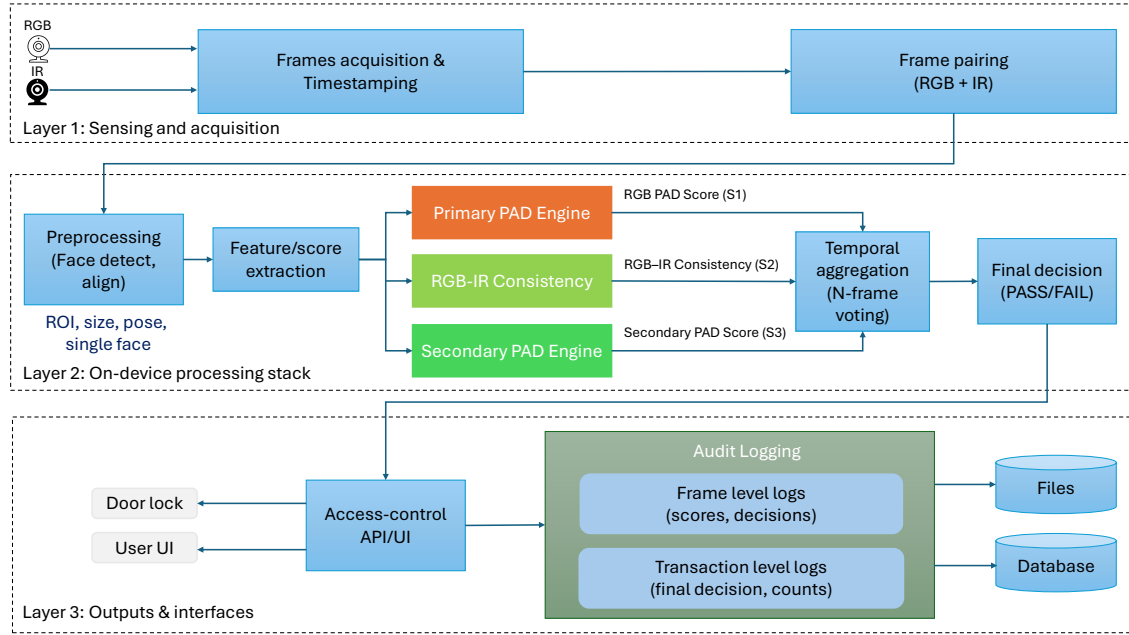
Fig. 2. On-device processing stack and data flow
