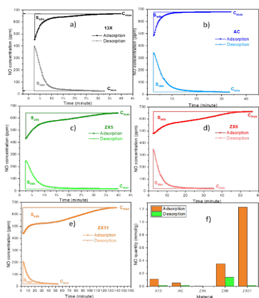
Fig. 7. NO adsorption and desorption curves of materials
