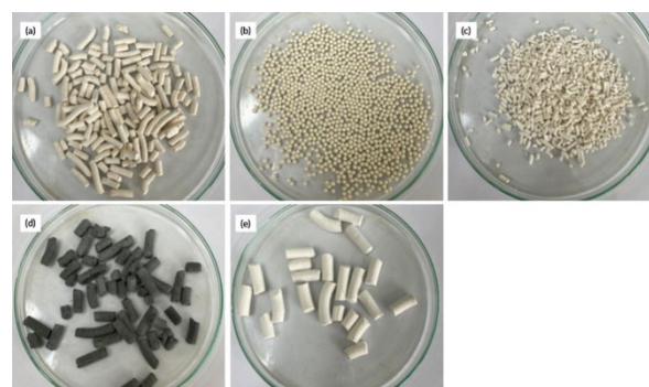
Fig. 1. Original shape of adsorbent materials: a) Zeolite ZX5 (zeolite 13X + 15% boehmite, pellets, 4 mm diameter, 0.6 - 1.2 cm length, calcination temperature: 610 °C); b) Zeolite 13X (zeolite 13X, sphere, 2 mm diameter, calcination temperature 400 °C); c) Zeolite ZX31 (zeolite 13X + 25% boehmite, pillars, 2 mm diameter, 0.25 - 0.6 cm length, calcination temperature 550 °C); d) Activated carbon (pellets, 5 mm diameter, 0.7 - 1.2 cm length); e) Zeolite ZX6 (zeolite 13X + 15% silica gel, pellets, 6mm diameter, 0.9 - 2 cm length, calcination temperature: 610 °C)
