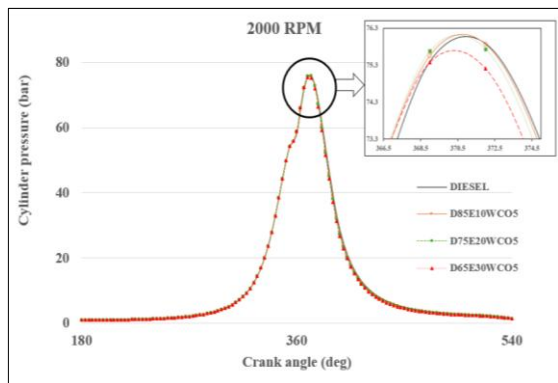
Fig. 8. Cylinder pressure at full load, 2000 rpm
