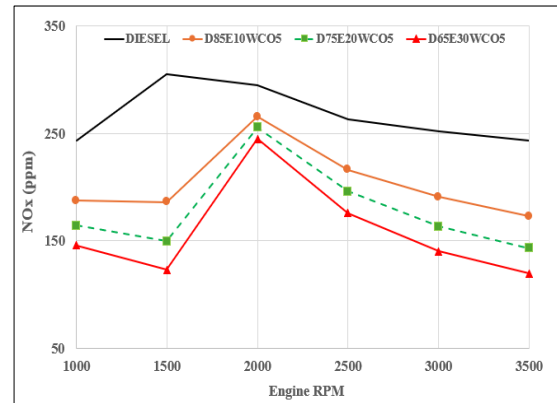
Fig. 16. NO x emissions at full load
