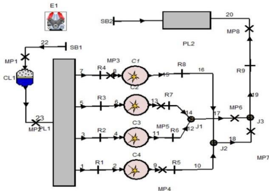
Fig. 1. Hyundai D4BB engine model
