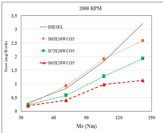
Fig. 19. Soot emissions at different loads, 2000 rpm
