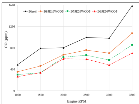
Fig. 14. CO emissions at full load
