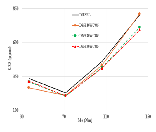
Fig. 15. CO emissions at different loads, 2000 rpm
