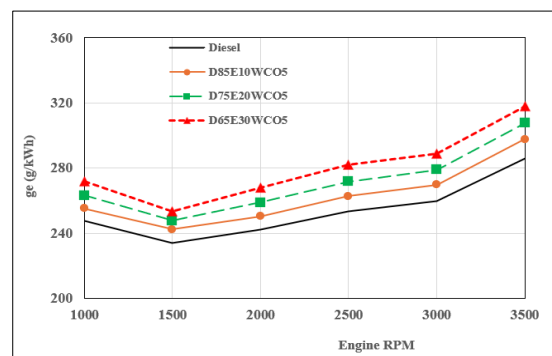
Fig. 6. Fuel consumption at full load
