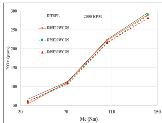
Fig. 17. NO x emissions at different loads, 2000 rpm
