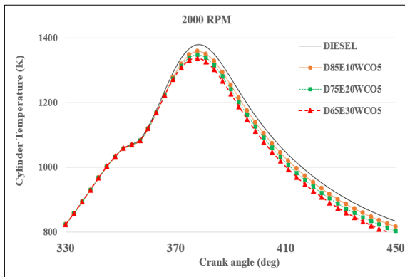
Fig. 13. Cylinder temperature at 36.56 Nm, 2000 rpm
