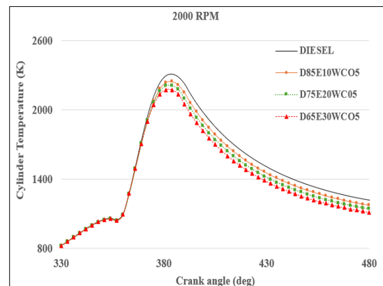
Fig. 12. Cylinder temperature at full load, 2000 rpm
