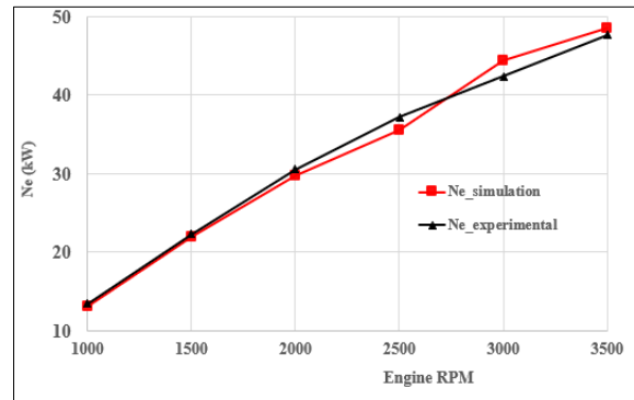
Fig. 2. Engine power at full load
