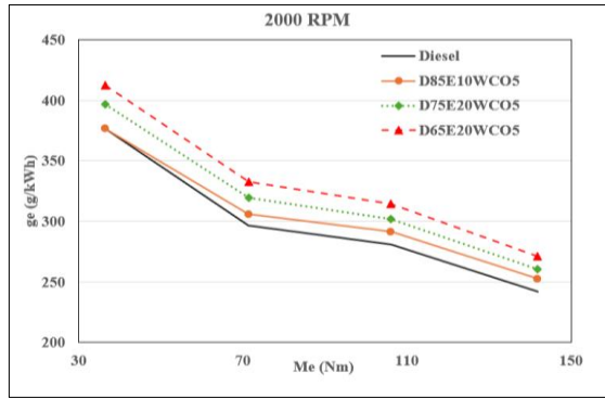
Fig. 7. Fuel consumption rate at different loads, 2000 rpm
