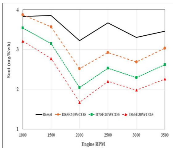
Fig. 18. Soot emissions at full load
