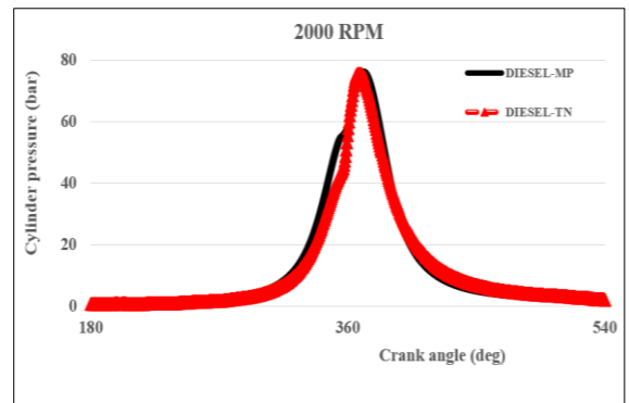
Fig. 3. Engine cylinder pressure at full load, 2000 rpm
