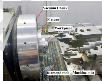
Fig. 5. Ultra-precision lathe system
