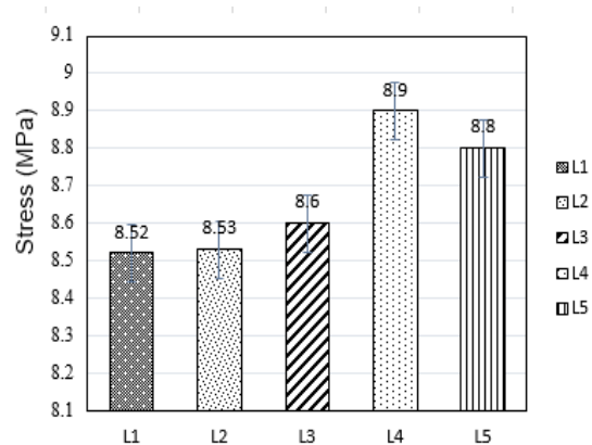
Fig. 7. Tensile strength of outsole material
