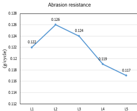
Fig. 13. Abrasion resistance of outsole material
