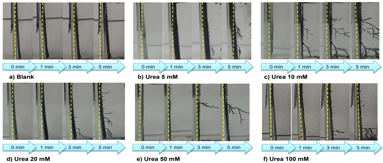
Fig. 5ne. In-situ optical images of initiation and growth process of zinc dendrites in the electrolyte (a) without and with urea additive at the different concentrations, (b) 5 mM, (c) 10 mM, (d) 20 mM, (e) 50 mM, and (f) 100 mM at a current of 1A
