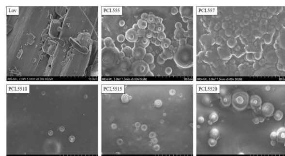
Fig. 4. FESEM images of pure Lov and PCL55x composites
