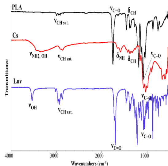
Fig. 2. FT-IR spectra of pure PLA , Cs , and Lov
