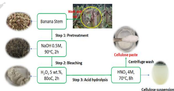
Fig. 1. Schematic illustration of the MFC extraction process from banana stem waste
