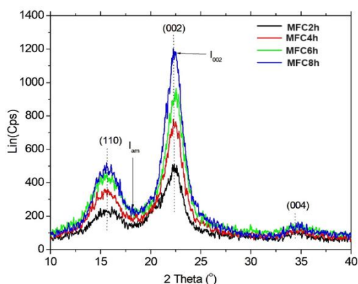
Fig. 4. XRD patterns of MFC samples at different alkali treatment times
