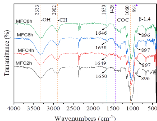
Fig. 5. FTIR spectra of MFC samples at different alkali treatment times
