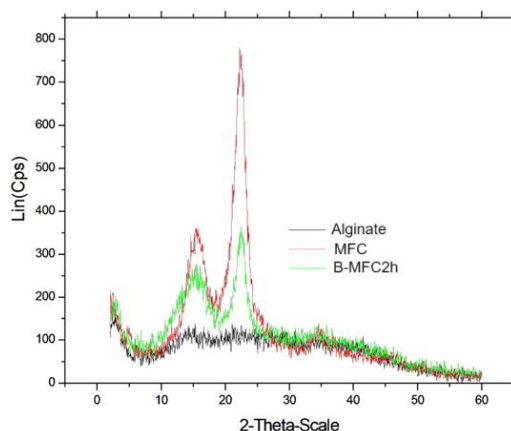
Fig. 7. XRD patterns of bio-hydrogel film and MFC samples
