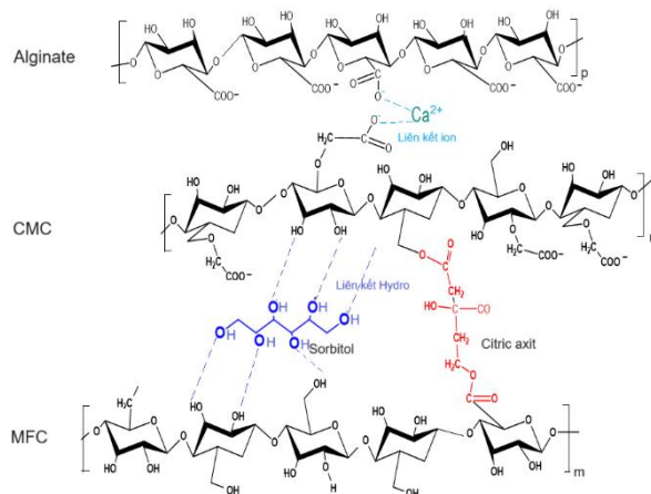
Fig. 2. Diagrammatic representation of the MFC-CMC-alginate hydrogel film's network creation
