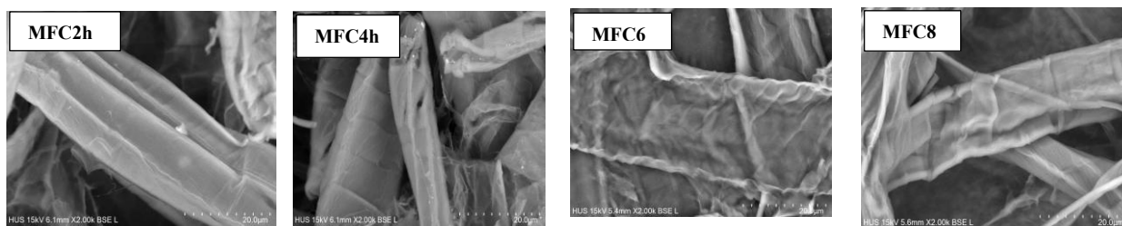
Fig. 3. SEM images of banana stem MFC samples at different alkali treatment times at 2000 x magnification (20 µm size bar)
