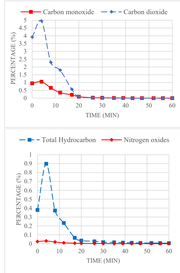
Fig. 4. Effluent gas composition during pyrolysis
