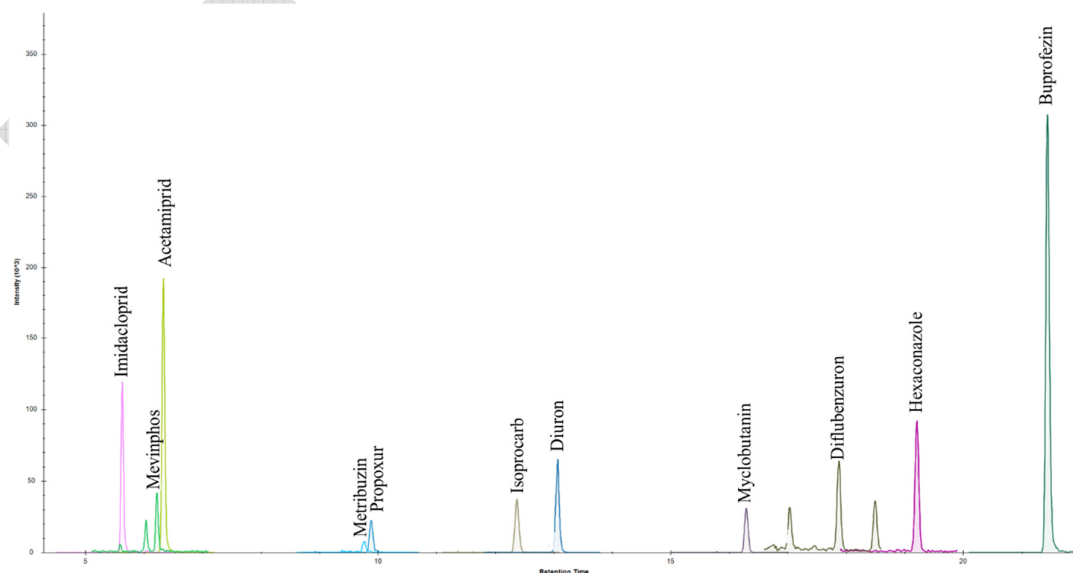
Fig. 1. UPLC-MS/MS chromatogram of 11 pesticides in standard solution
