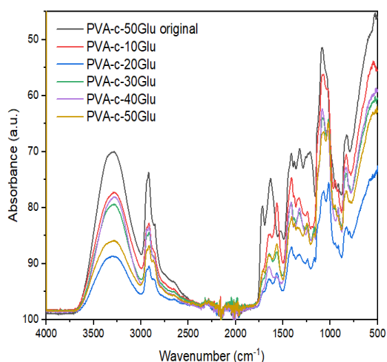
Fig. 9. FT-IR spectra of the original PVA-c-50Glu material and PVA-c-x%Glu material after biodegradation
