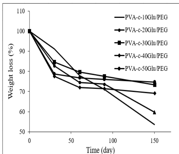
Fig. 6. Mass loss graph of PVA-c-x%Glu/PEG material during biodegradation in natural soil
