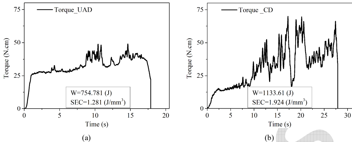
Fig. 7. Energy efficiency comparison: (a) UAD, (b) CD
