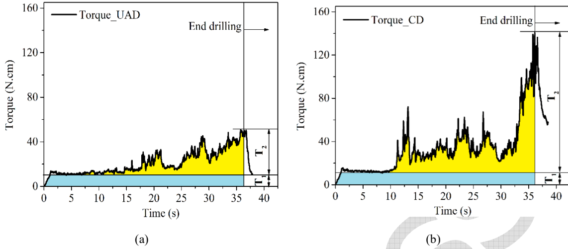
Fig. 2. Torque measured while drilling at the same cutting conditions ( n = 1000 rpm and f = 0.05 mm/rev): (a) UAD and (b) CD
