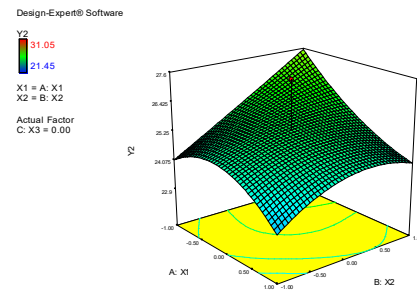
Fig. 6. The response of the elongation of the sealing seam before aging - Y_2 (%) at different levels of sealing temperature - X_1 (°C) and sealing speed - X_2 (m/min)
