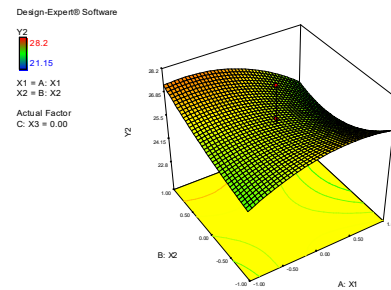
Fig. 12. The response of the elongation of sealing seam after aging - Y_2 (%) at different levels of sealing temperature - X_1 ( ^{\circ}\text{C} ) and sealing speed - X_2 (m/min)
