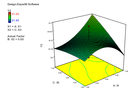
Fig. 7. The response to the elongation of the sealing seam before aging - Y_2 (%) at different levels of sealing temperature - X_1 (°C) and roller pressure - X_3 (MPa)
