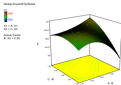
Fig. 10. The response of sealing seam tensile strength after aging Y_1 (N) at different levels of sealing temperature - X_1 (°C) and roller pressure - X_3 (MPa)
