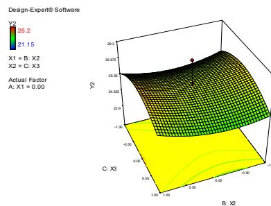
Fig. 14. The response of the elongation of sealing seam after aging - Y_2 (%) at different levels of Sealing speed - X_2 (m/min) and roller pressure - X_3 (m/min)
