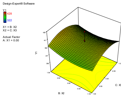
Fig. 11. The response of sealing seam tensile strength after aging - Y_1 (N) at different levels of sealing speed - X_2 (m/min) and roller pressure - X_3 (MPa)
