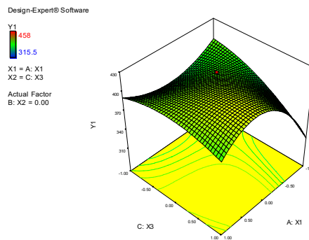
Fig. 4. The response of sealing seam tensile strength before aging - Y_1 (N) at different levels of sealing temperature - X_1 ( ^{\circ}\text{C} ) and roller pressure - X_3 (MPa)
