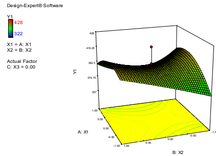
Fig. 9. The response of sealing seam tensile strength after aging Y_1 (N) at different levels of sealing temperature - X_1 (°C) and Sealing speed - X_2 (m/min)
