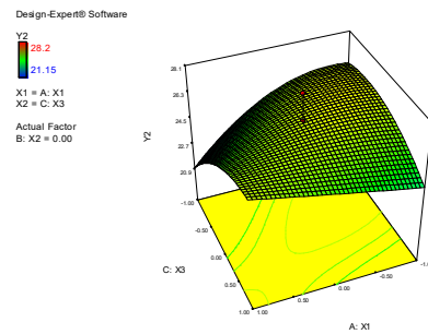
Fig. 13. The response of the elongation of sealing seam after aging - Y_2 (%) at different levels of sealing temperature - X_1 ( ^{\circ}\text{C} ) and roller pressure - X_3 (MPa)
