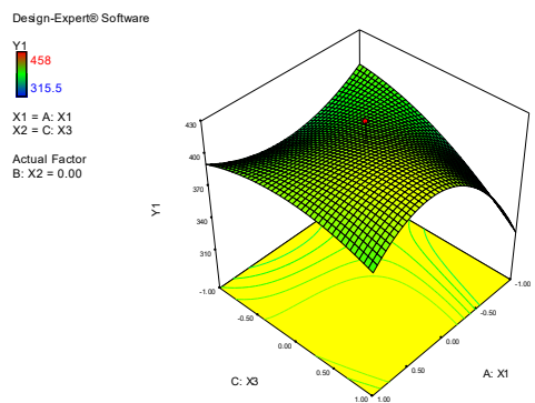
Fig. 4. The response of sealing seam tensile strength before aging - Y_1 (N) at different levels of sealing temperature - X_1 ( ^{\circ}\text{C} ) and roller pressure - X_3 (MPa)
