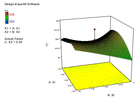
Fig. 9. The response of sealing seam tensile strength after aging Y_1 (N) at different levels of sealing temperature - X_1 (°C) and Sealing speed - X_2 (m/min)
