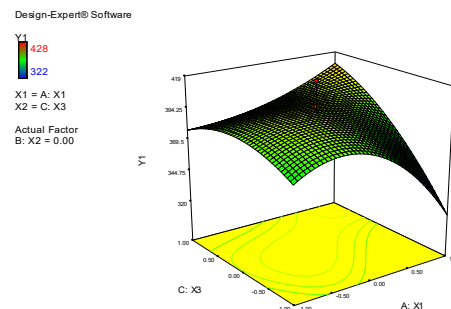
Fig. 10. The response of sealing seam tensile strength after aging Y_1 (N) at different levels of sealing temperature - X_1 (°C) and roller pressure - X_3 (MPa)
