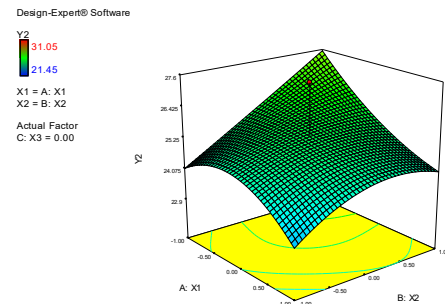
Fig. 6. The response of the elongation of the sealing seam before aging - Y_2 (%) at different levels of sealing temperature - X_1 (°C) and sealing speed - X_2 (m/min)
