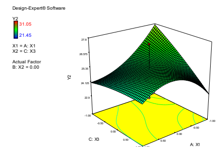
Fig. 7. The response to the elongation of the sealing seam before aging - Y_2 (%) at different levels of sealing temperature - X_1 (°C) and roller pressure - X_3 (MPa)
