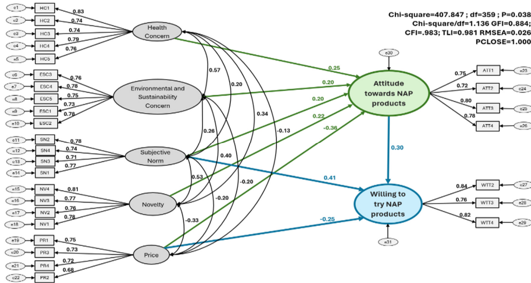
Fig. 3. Standardized SEM model
