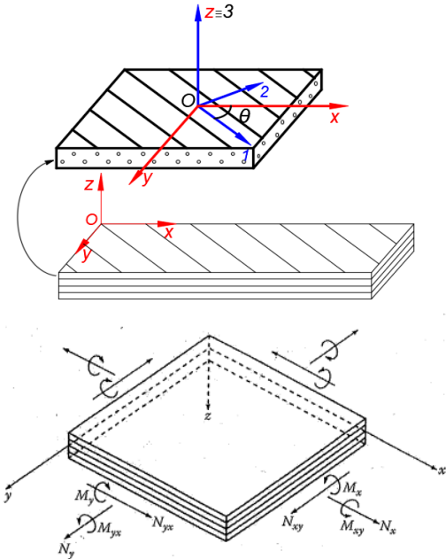
Fig. 1. Coordinate systems, forces and moments acting on laminate
