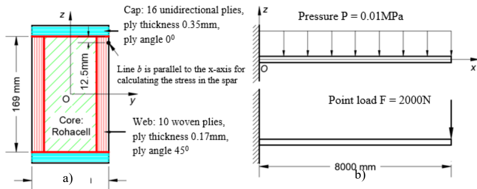
Fig. 2. Cross section of beam and load applied to it
