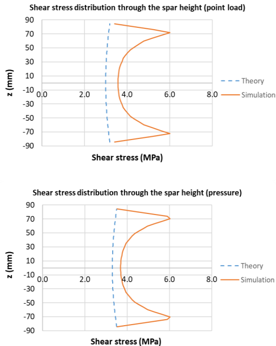
Fig. 8. The variation of shear stress in the beam web along the z -coordinate
