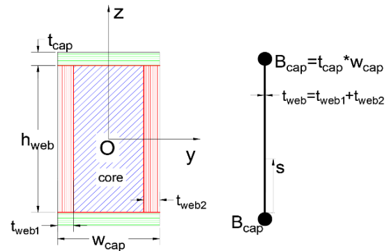
Fig. 3. Idealization of the cross-section of the beam
