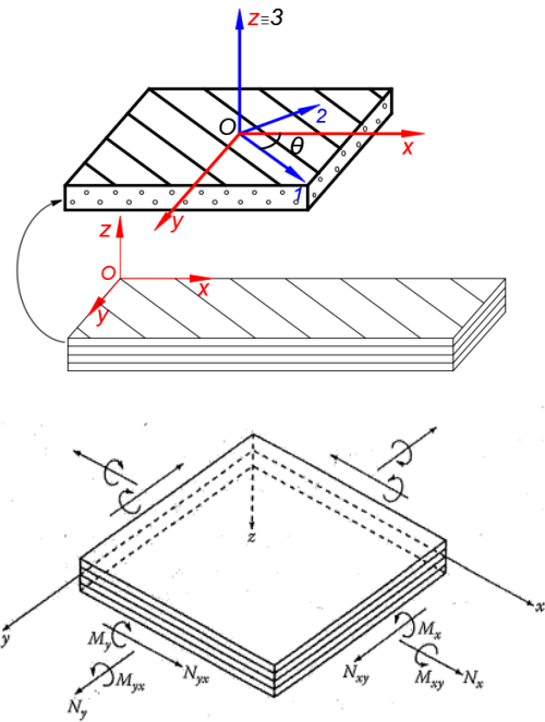
Fig. 1. Coordinate systems, forces and moments acting on laminate
