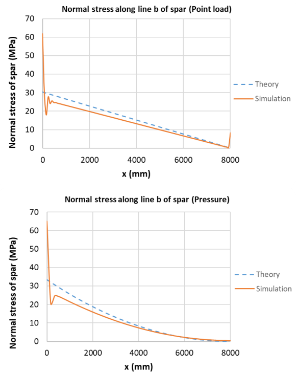
Fig. 7. Normal stress on the line b of the web
