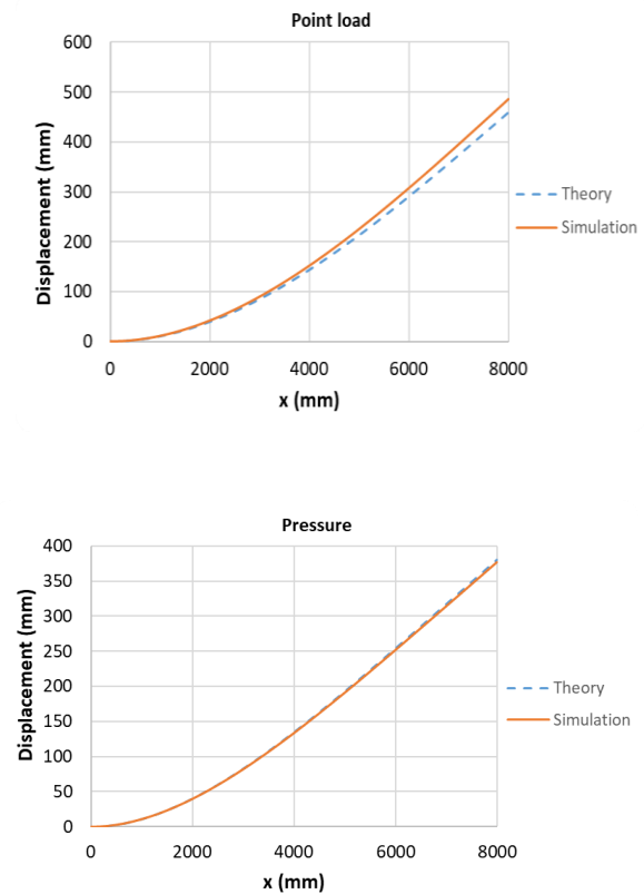
Fig. 4. Displacement along the beam under two loading conditions
