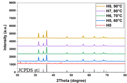
Fig. 4. XRD patterns of ZnO NMs samples
