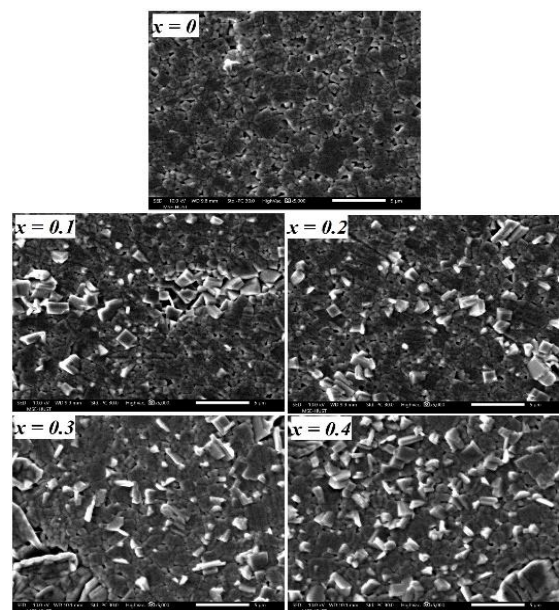
Fig. 5. SEM microstructure of the BNBT- x STN ceramics with x equal to 0–0.4
