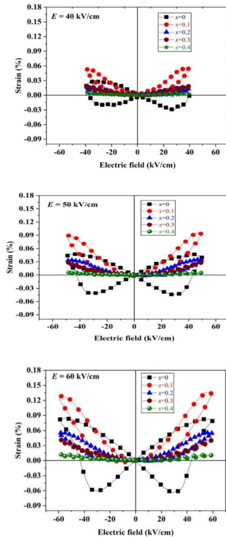
Fig. 7. Electric field-induced strain ( S - E ) of BNBT- x STN ceramics at different electric fields
