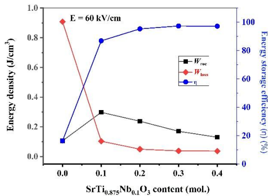
Fig. 14. W_{rec} , W_{loss} and \eta of BNBT-STN samples as a function of x under an applied electric field of 60 kV/cm
