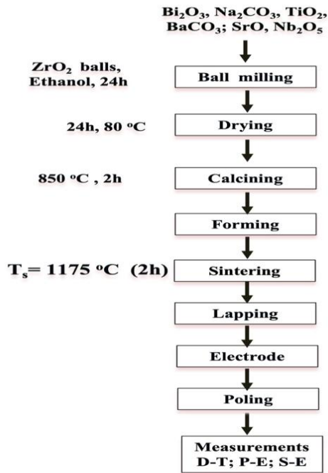
Fig. 1. Experimental procedure of BNBT- x STN bulk ceramic
