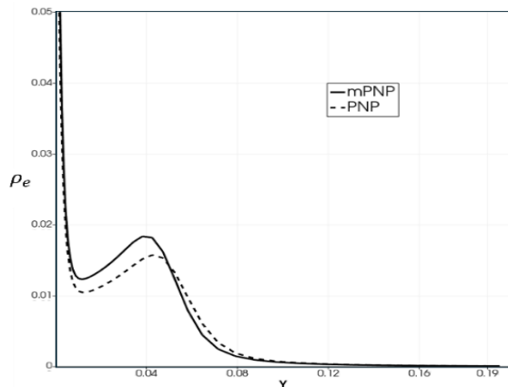
Fig. 8. Comparison of the ESC profile near the electrode in overlimiting regimes: with and without steric effects at V equal 30 V_0
