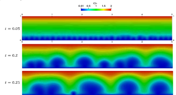
a) The ion distribution follows the PNP-NS equations ( v = 0 )
