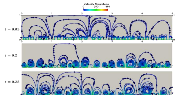
b) The ion distribution follows the mPNP-NS equations ( v = 0.01 )
