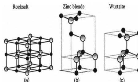
Fig. 1. ZnO crystal structures: simple cubic NaCl-type lattice (a), cubic zinc blende-type lattice (b), and hexagonal wurtzite lattice (c) [3]
