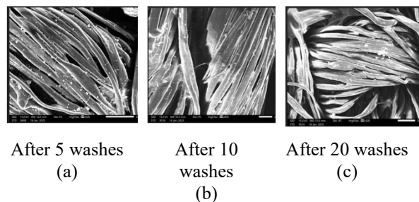
Fig. 16. SEM of Ag-doped ZnO nano-coated cotton fabric after washes
