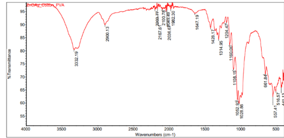
Fig. 15. FTIR analysis of Ag-doped ZnO-coated cotton fabric
