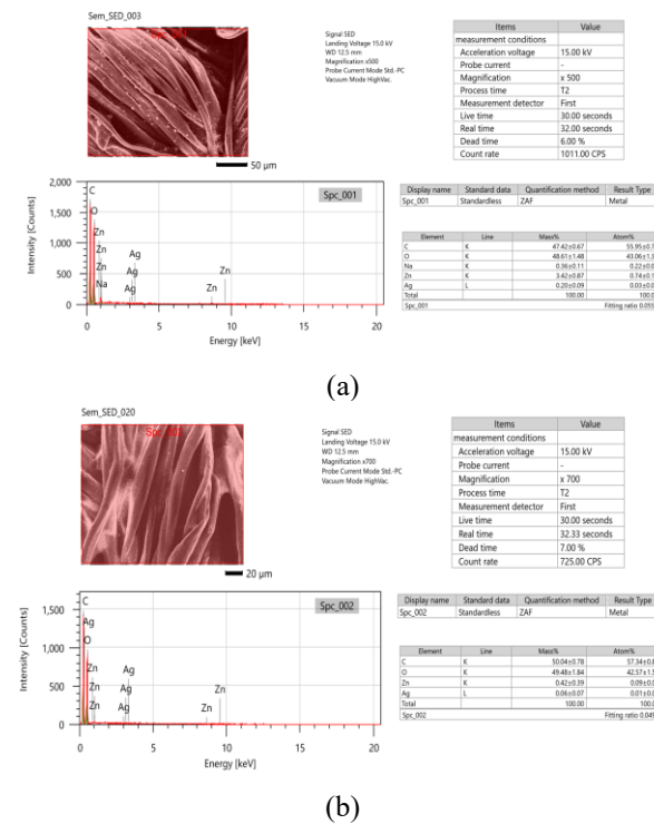
Fig. 17. EDS of of nano Ag-doped zinc oxide coated on cotton fabric before washing (a) and after 20 washes (b)
