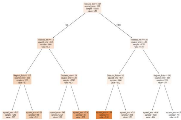
Fig. 9. Selection logic
