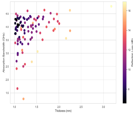
Fig. 4. Bandwidth sensitivity
