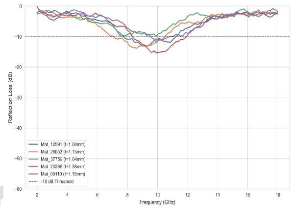
Fig. 6. Performance curves
