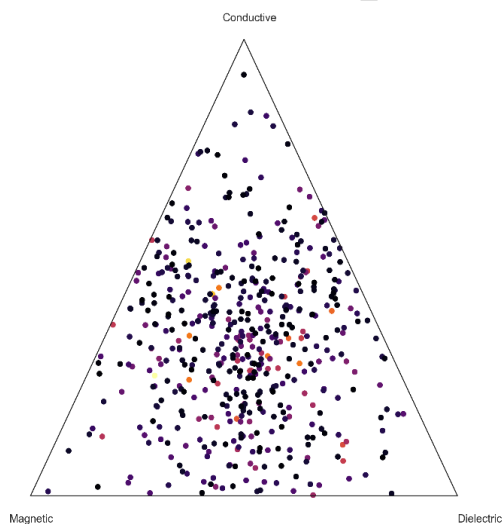
Fig. 5. Stoichiometry
