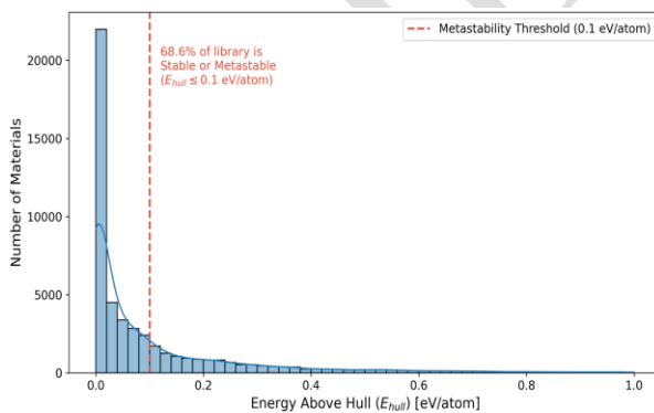
Fig. 1. Distribution of thermodynamic stability (Energy above hull)
