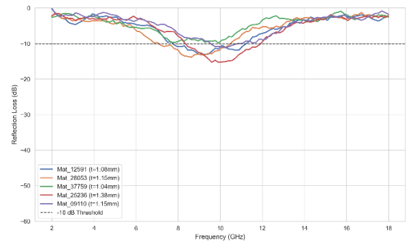
Fig. 6. Performance curves
