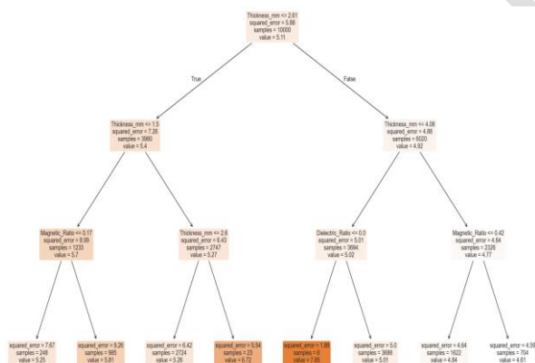
Fig. 9. Selection logic
