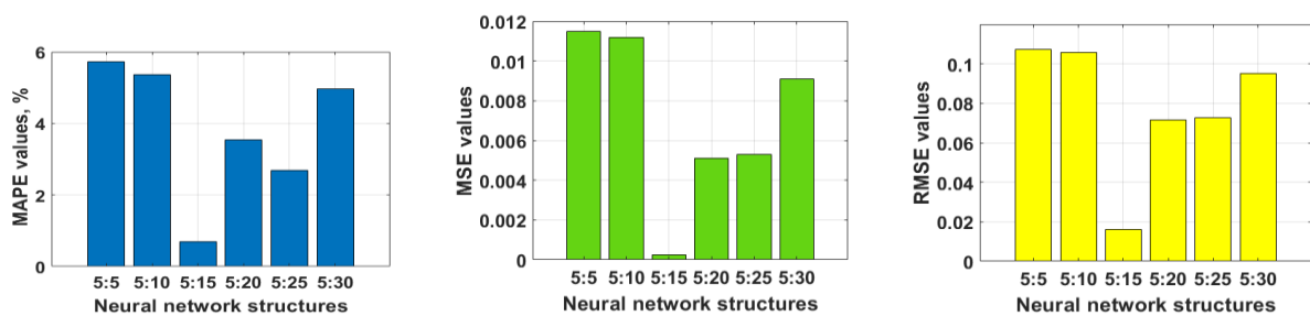
Fig. 7. MSE , RMSE , MAPE values corresponding to the structure ratios
