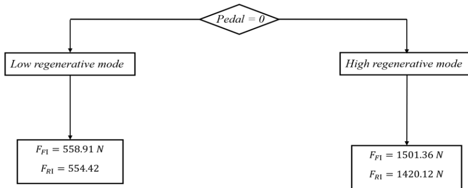
Fig. 5. Control algorithm logic of braking force distribution between front axle and rear axle at pedal equal 0
