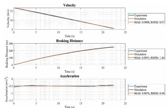
Fig. 11. Low-regenerative mode (60 km/h)
