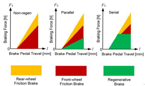
Fig. 3. Three different control strategies for regenerative braking
