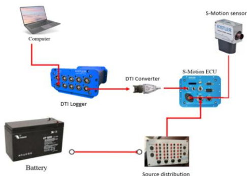
Fig. 8. Connection diagram
