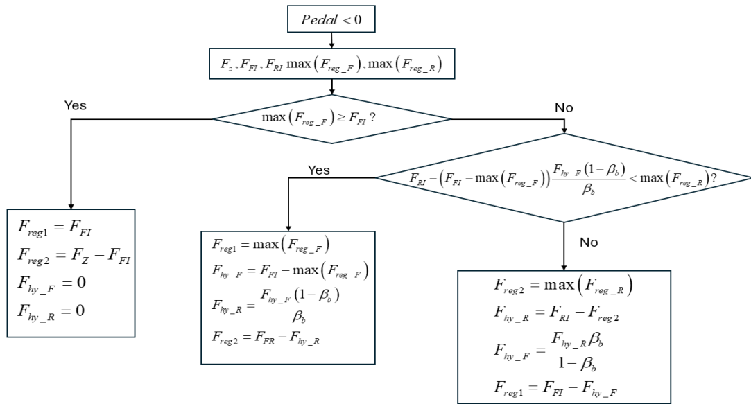
Fig. 4. Control algorithm logic of braking force distribution between front axle and rear axle at pedal signal under 0
