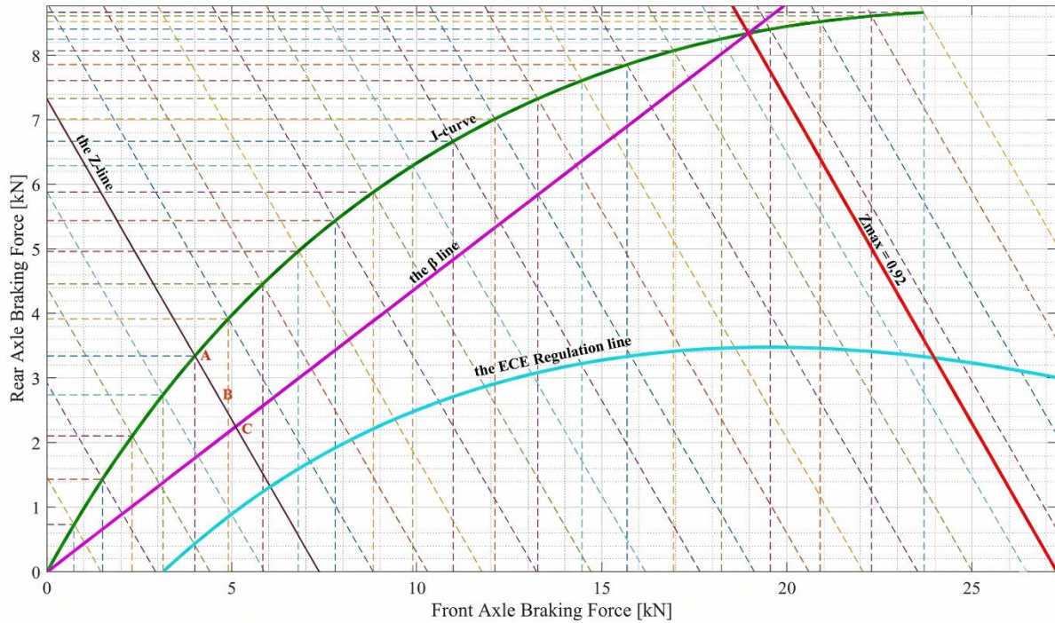
Fig. 2. Braking force distribution strategy based on I-curve I [7]
