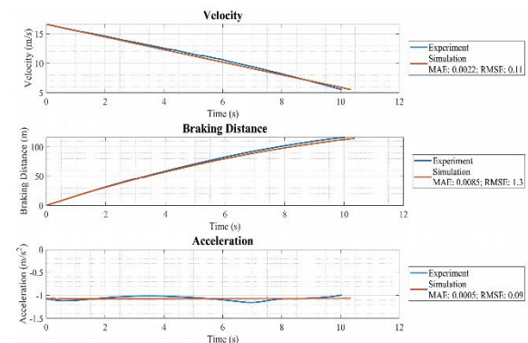
Fig. 12. High-regeneration mode (at 60 km/h)
