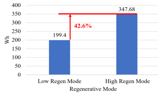
Fig. 15. Regenerative energy in rush hours driving cycle in Vietnam
