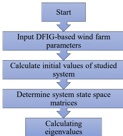
Fig. 4. Calculating eigenvalues flowchart
