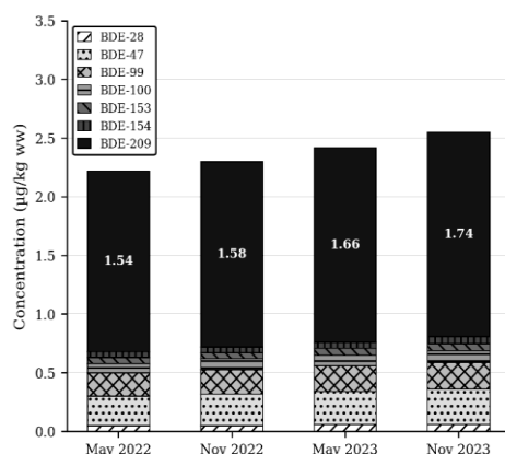
Fig. 2. Stacked bar chart of mean PBDE congener concentrations ( \mu\text{g/kg ww} ) across four sampling periods from West Lake, Hanoi
