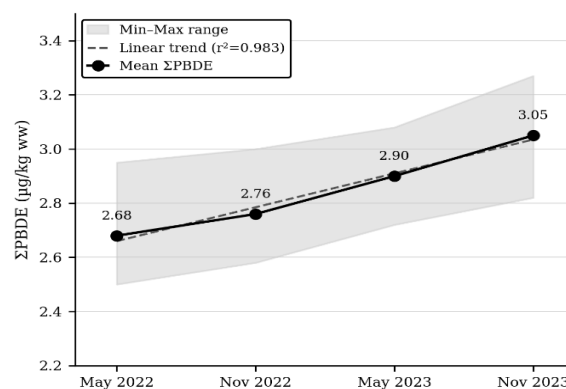
Fig. 3. Temporal trend of \Sigma PBDE concentrations in snail samples from West Lake, Hanoi (May 2022 – Nov 2023). Shaded band: observed min-max range; dashed line: linear trend ( n = 10 per period)
