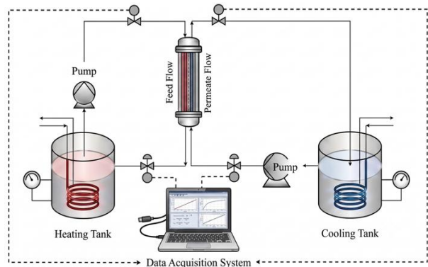
Fig. 2. DCMD system setup
