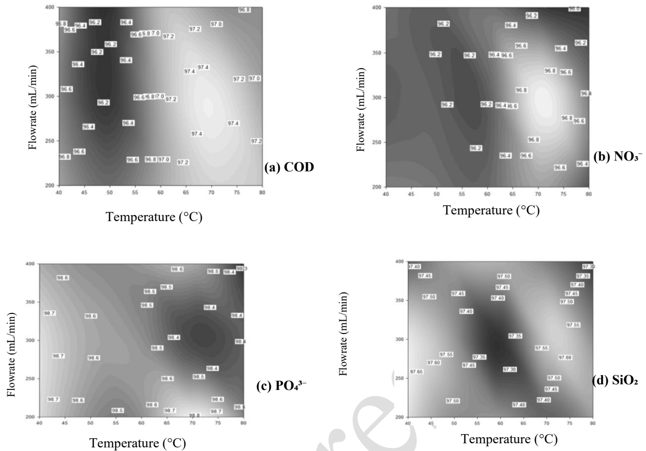
Fig. 5. Pollutant removal efficiency under the investigated conditions (a) COD; (b) NO 3 - ; (c) PO 4 3- ; (d) SiO 2
