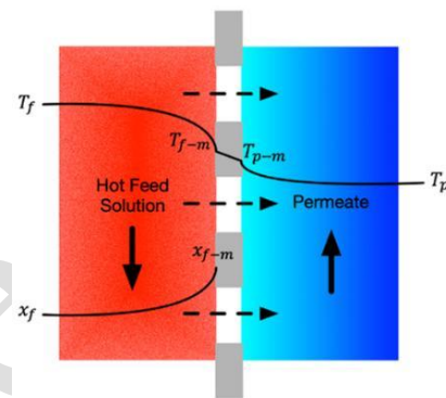
Fig. 1. Operating principle of DCMD
