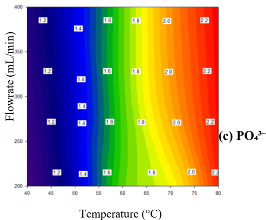
Fig. 4. Concentration factors of nutrients under the investigated conditions. (a) COD; (b) \text{NO}_3^- ; (c) \text{PO}_4^{3-} ; (d) \text{SiO}_2
