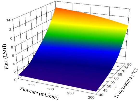
Fig. 3. Influence of temperature and flow rate on permeate flux
