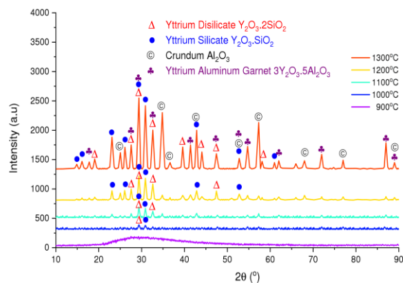
Fig. 4. XRD patterns of 2A5Y2S frit fired for 0.5 hours at (a) 900^\circ\text{C} , (b) 1000^\circ\text{C} , (c) 1100^\circ\text{C} , (d) 1200^\circ\text{C} , and (e) 1300^\circ\text{C}
