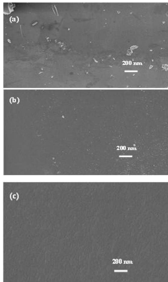
Fig. 8. SEM image of 2A4Y3S frit melted at 1200^\circ\text{C} for (a) 0.5 hours, (b) 5 hours, and (c) 10 hours
