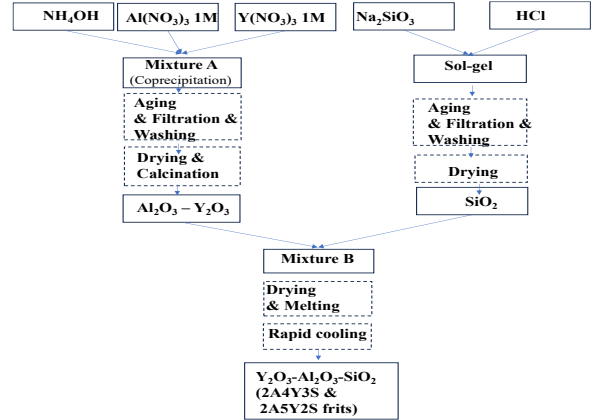
Fig. 1. Synthesis process of 2A4Y3S and 2A5Y2S frits
