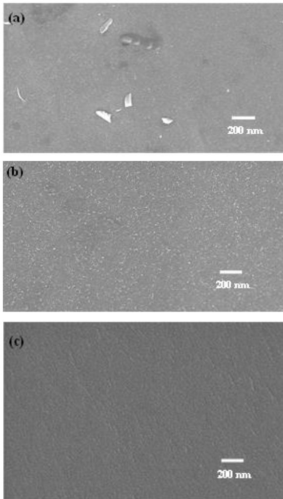
Fig. 9. SEM image of 2A5Y2S frit melted at 1300 °C for (a) 0.5 hours (b) 5 hours and (c) 10 hours
