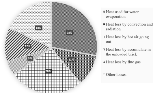
Fig. 2. Distribution of heat loss sources based on the Energy balance for the case of the investigated multi-chamber kiln.
