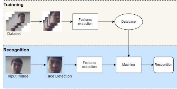
Fig. 3. Facial recognition-based patient identification process
