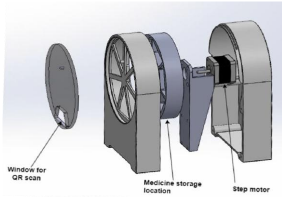
Fig. 6. 3D structure of the medication dispensing device
