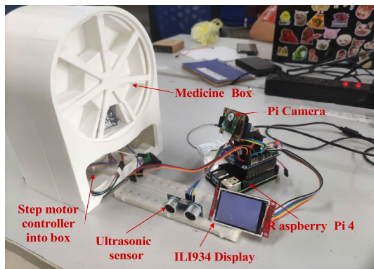
Fig. 7. Final product of the automated medication dispensing device
