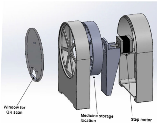
Fig. 6. 3D Structure of the medication dispensing device
