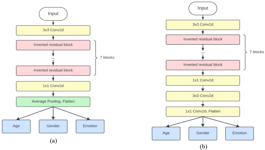
Fig. 1. Multi-task CNN architecture of the proposed system: a) MobileNetV2 backbone (left), b) customized MobileNetV2 (right)
