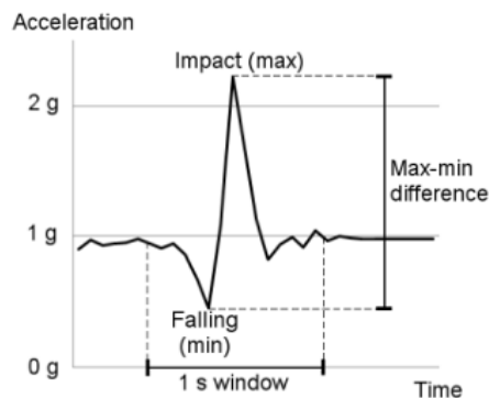
Fig. 10. Acceleration graph when falling
