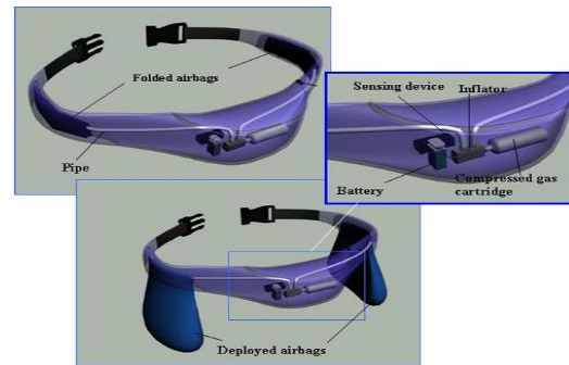
Fig. 2. Conceptual illustration of the “intelligent” human airbag system
