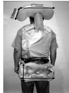
Fig. 3. Airbag system
