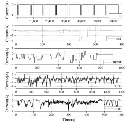
Fig. 6. Input currents in each experiment in one cycle
