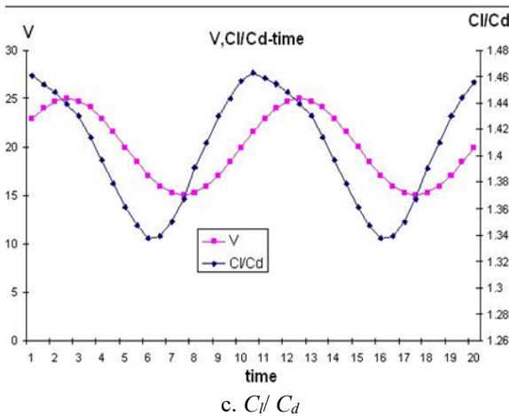
Fig. 7. Aerodynamic characteristics of UAV – V_0 = 20 m/s and f = 0.1 Hz.
