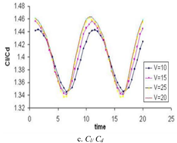
Fig. 8. Aerodynamic characteristics of UAV – Effect of V_0 at f = 0.1 Hz.
