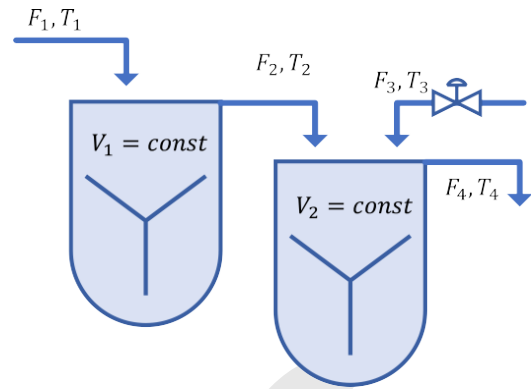
Fig. 1. Studied dual-tank mixing system configuration
