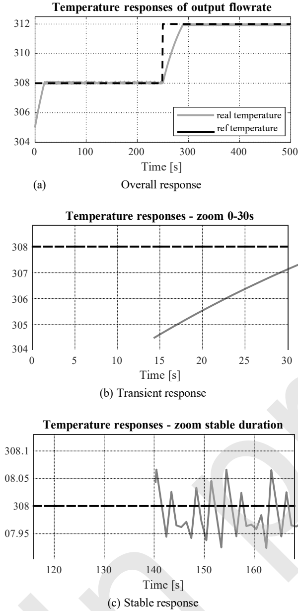
Fig. 5. Temperature response with DDPG algorithm
