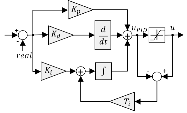
Fig. 7. Anti-windup PID controller with back-calculation method
