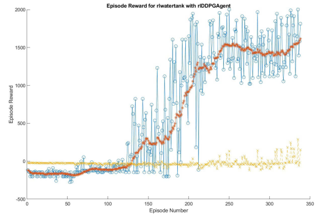
Fig. 4. Training process of agent
