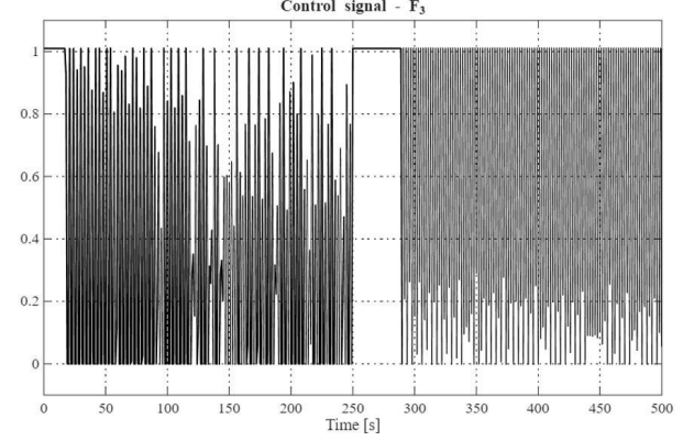
Fig. 6. Control signal F_3(t) under DDPG illustrating the respecting valve limits of DDPG command
