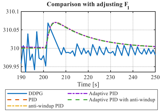
Fig. 9. Comparison result of T_4 with disturbance F_1
