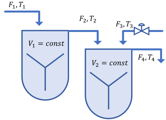
Fig. 1. Studied dual-tank mixing system configuration
