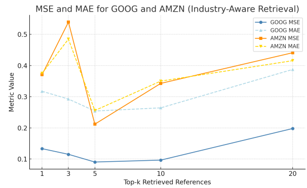
Fig. 4. Effect of Top- k retrieved references on IA-RATD performance. Solid lines denote MSE, dashed lines denote MAE. The optimal point occurs near k = 5 , balancing diversity and relevance
