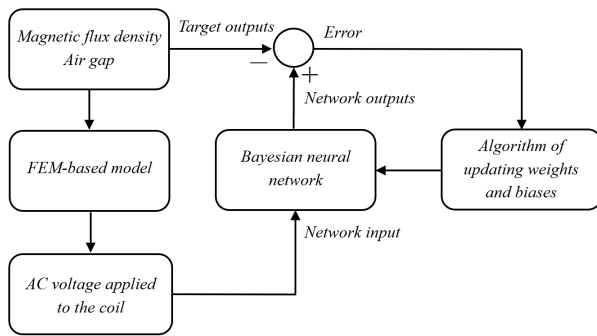
Fig. 6. Principle for updating the weights and biases of the BNN
