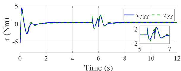
Fig. 5. Control signal
