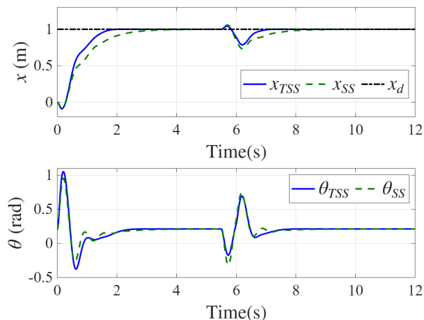
Fig. 4. State response
