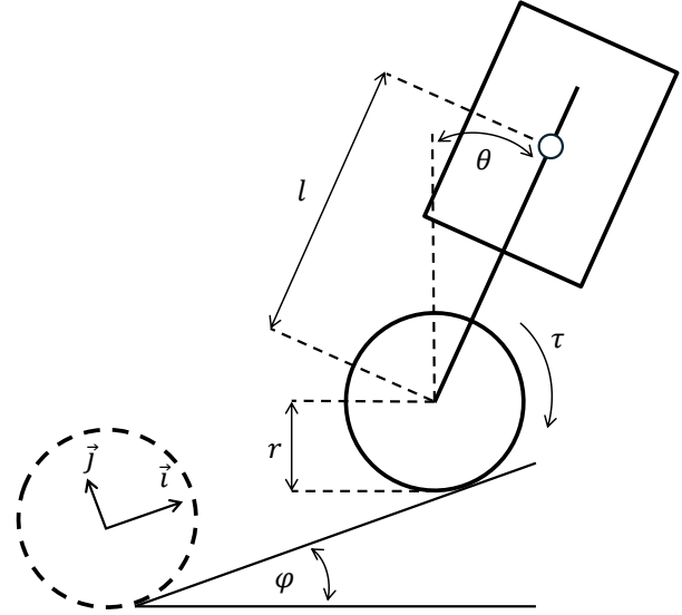
Fig. 1. Upright model in 2D
