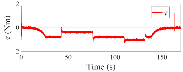
Fig. 11. Control signal
