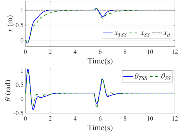
Fig. 4. State response
