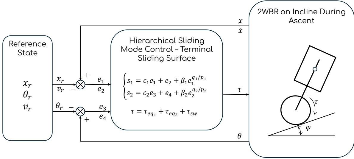
Fig. 3. Control structure
