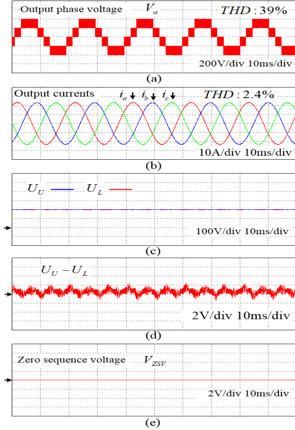
Fig. 9. Simulation results of the proposed SVM method at m = 0.8 : (a), output phase voltage V_a , (b), output currents i_a , i_b , i_c , (c) capacitor voltages U_U , U_L , (d) neutral-point voltage U_U - U_L , and (e), ZSV component V_{ZSV}
