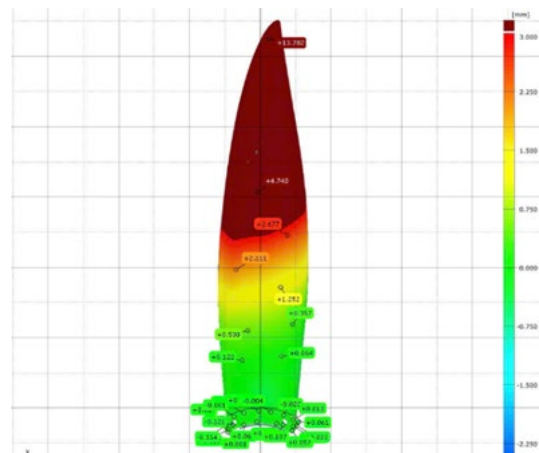
Fig. 28. Results of the comparison between the 3D scan of the physical sample and CAD file
