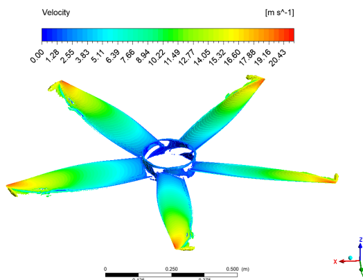
Fig. 22. Velocity field at the surface
