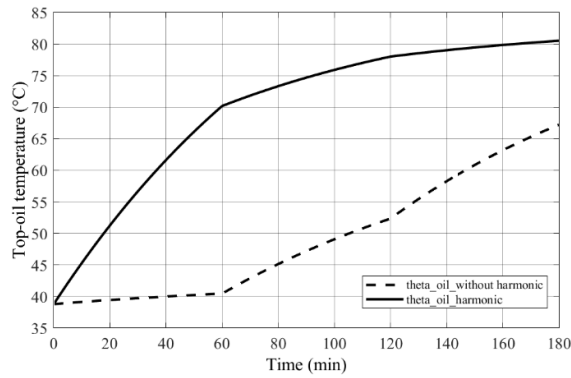
Fig. 9. Top-oil temperature
