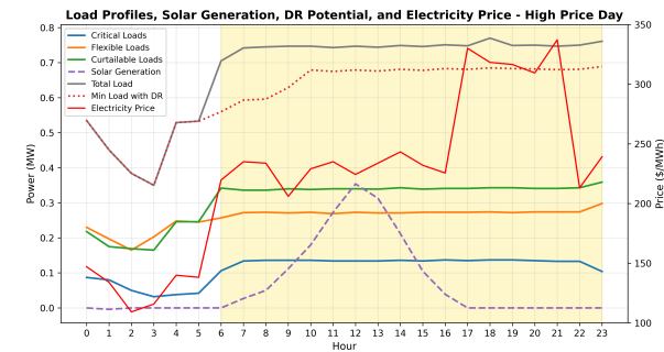
Fig. 4. Data analysis of March 31, 2015 (high price day)
