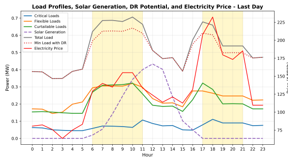
Fig. 2. Data analysis of September 15, 2015 (last day)
