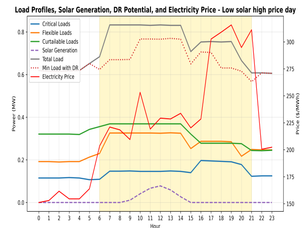
Fig. 10. Data analysis of February 6, 2015 (low solar high price)
