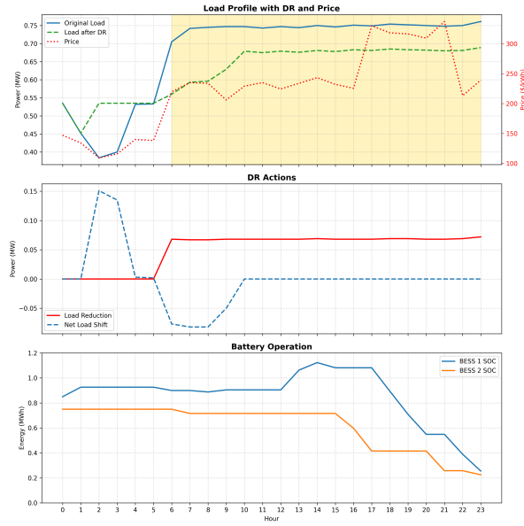
Fig. 5. Optimization results of March 31, 2015 (high price day)
