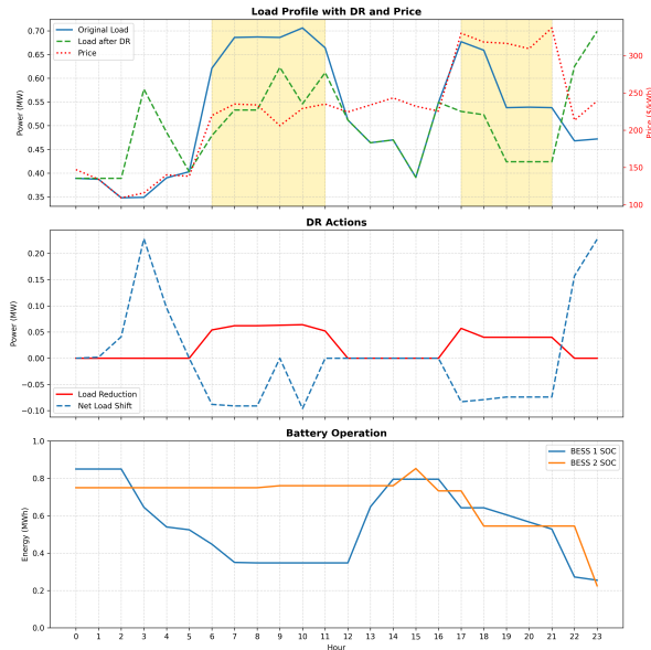
Fig. 3. Optimization results of September 15, 2015 (last day)
