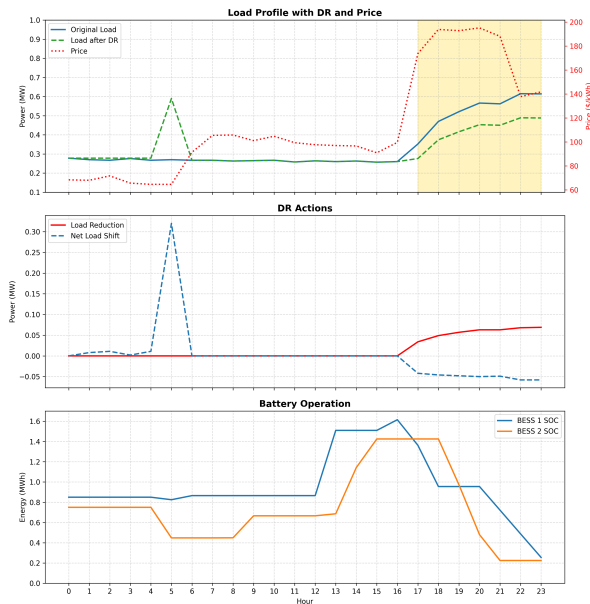
Fig. 9. Optimization results of August 19, 2015 (high solar low price)
