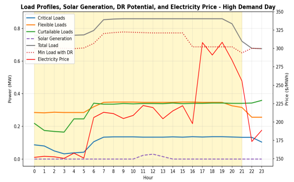
Fig. 6. Data analysis of December 30, 2014 (high demand day)
