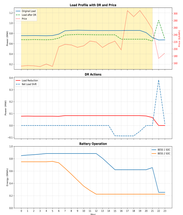
Fig. 7. Optimization results of December 30, 2014 (high demand day)
