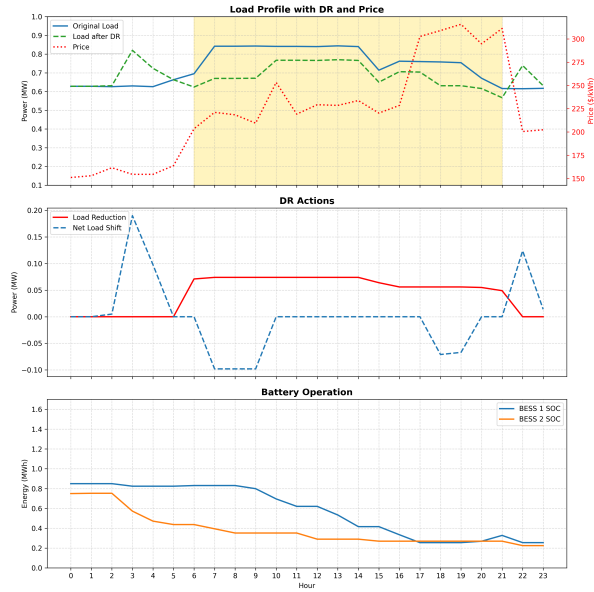
Fig. 11. Optimization results of February 6, 2015 (low solar high price)
