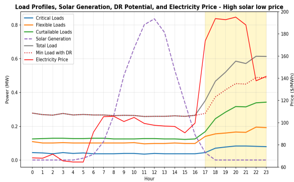
Fig. 8. Data analysis of August 19, 2015 (high solar low price)
