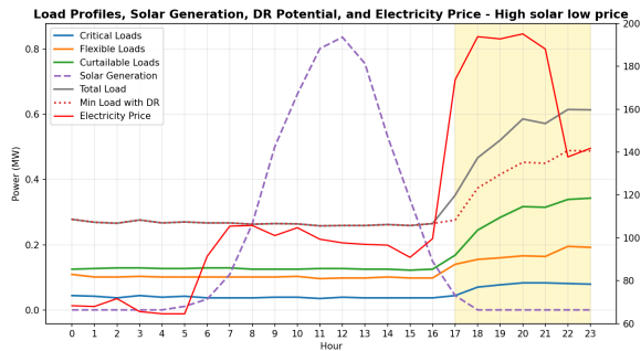
Fig. 8. Data analysis of August 19, 2015 (high solar low price)
