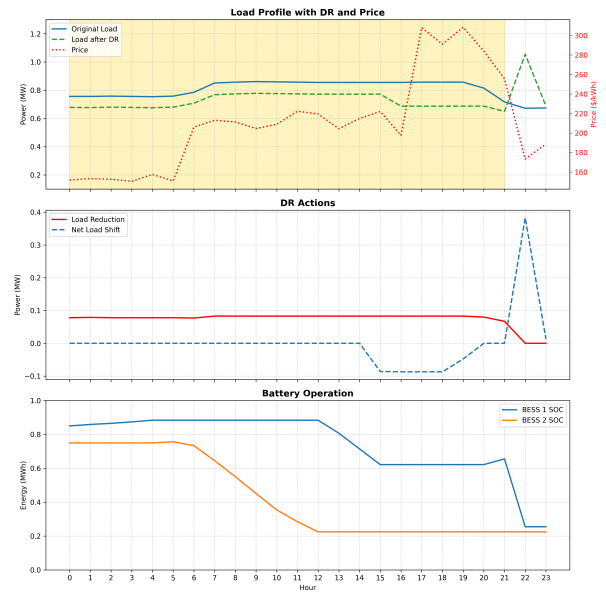
Fig. 7. Optimization results of December 30, 2014 (high demand day)
