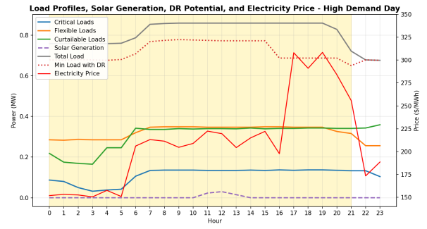
Fig. 6. Data analysis of December 30, 2014 (high demand day)
