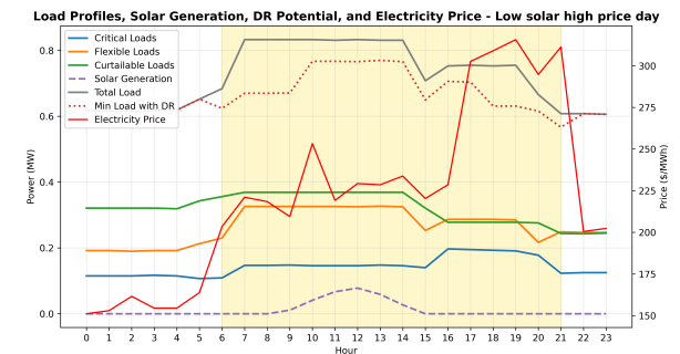
Fig. 10. Data analysis of February 6, 2015 (low solar high price)
